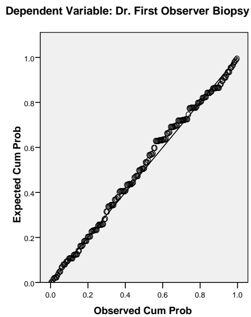
Figure 3: Regression line Fitting the data of observer one without intercept
